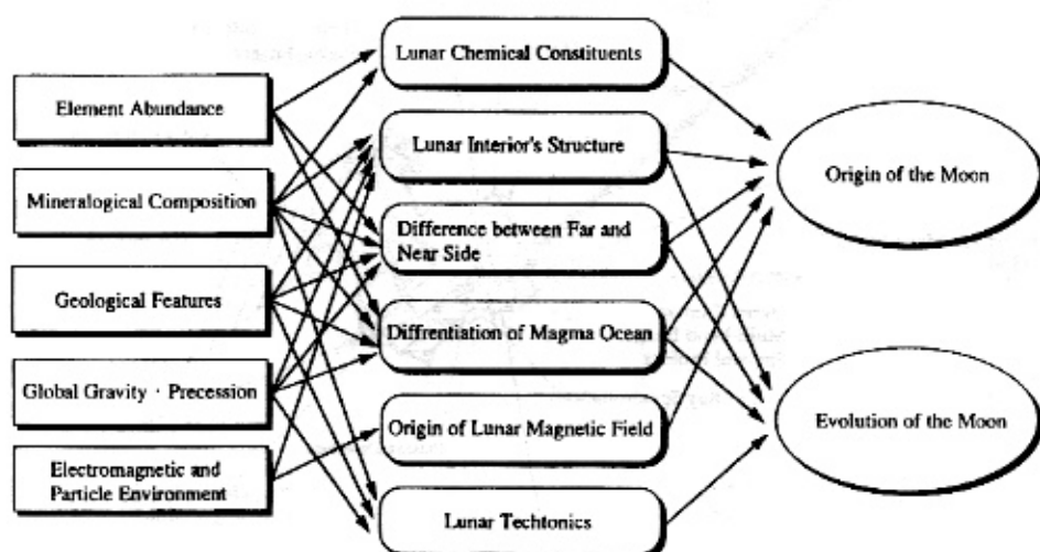
Figure 3 Integrated Research Scenario towards the Origin and Evolution of the Moon.
