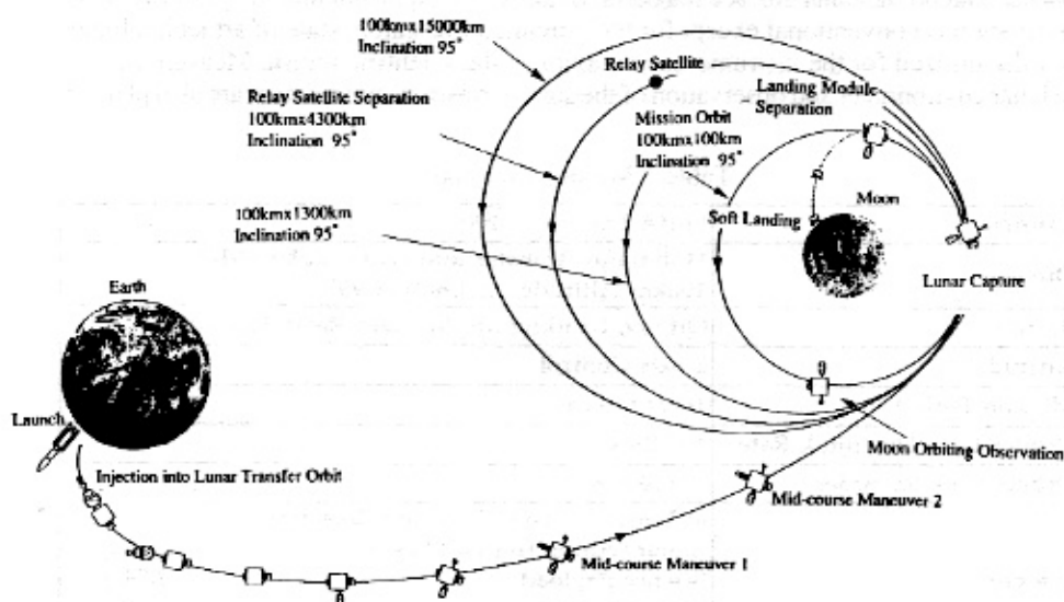
Figure 1 SELENE Mission Profile.
