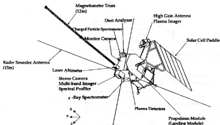
Figure 2 Concept of SELENE Orbiter Configuration.
